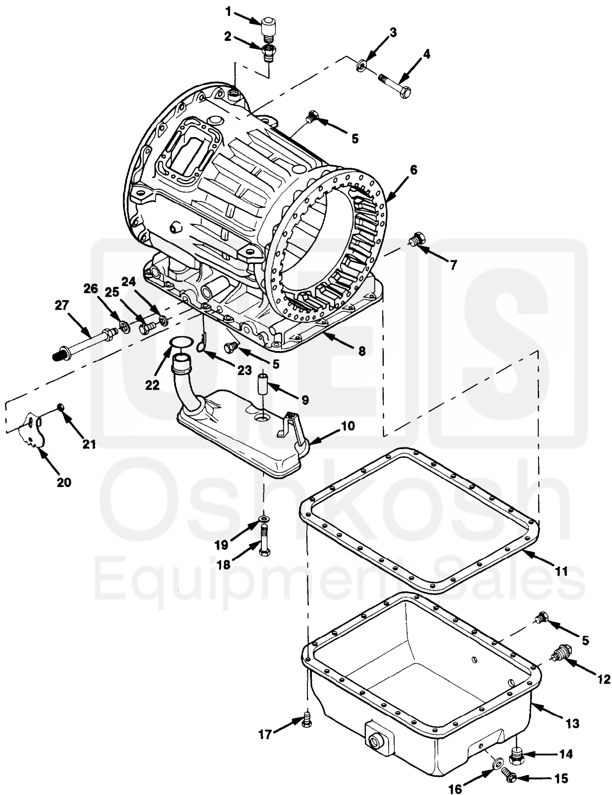
Figure 101. Transmission Housing, Oil Filter, and Oil Pan
